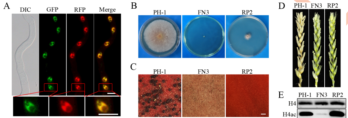
Fig 8. Localization of FgRpd3 and phenotypes of the FgRpd3 deletion mutant. (A). Germlings of the FNG1 -GFP FgRpd3 -RFP transformant (FCRR1) were examined by DIC and epifluorescence microscopy. The lower panels are close-up view of the indicated nuclei. Bar, 5 \mu m. (B). Three-day-old PDA cultures of PH-1, fng1 mutant (FN3), and FgRpd3 mutant (RP2). (C). 8 days post-fertilization (dpf) mating cultures of the indicated strains. Bar, 1 mm. (D). Flowering wheat heads inoculated with PH-1, FN3, and RP2 were photographed at 14 dpi. Black dots mark the inoculated spikelets. (E). Western blots of total proteins isolated from PH-1, FN3, and RP2 were detected with an anti-H4ac antibody. Detection with the anti-H4 antibody was used as a loading control.
